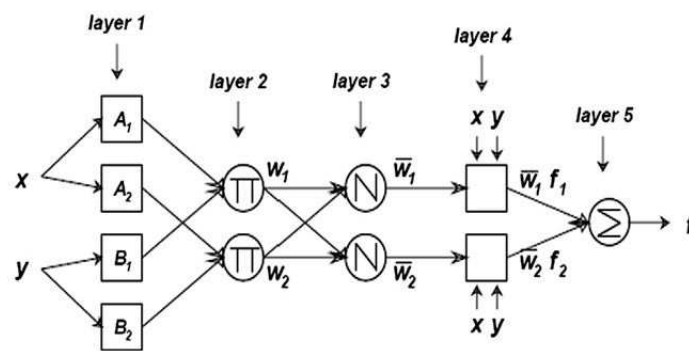
FIGURE 1. Architecture of ANFIS structure
