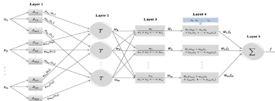
FIGURE 2. Schematic structure of ANFIS network
