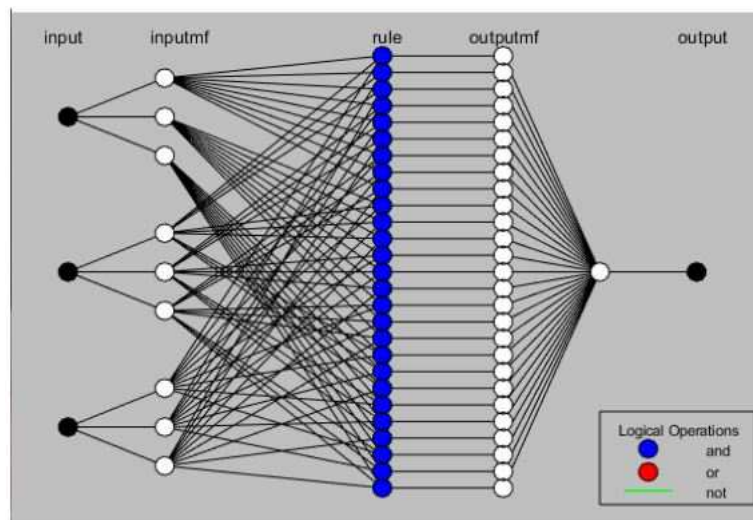
FIGURE 3. ANFIS Structure based on grid partition
